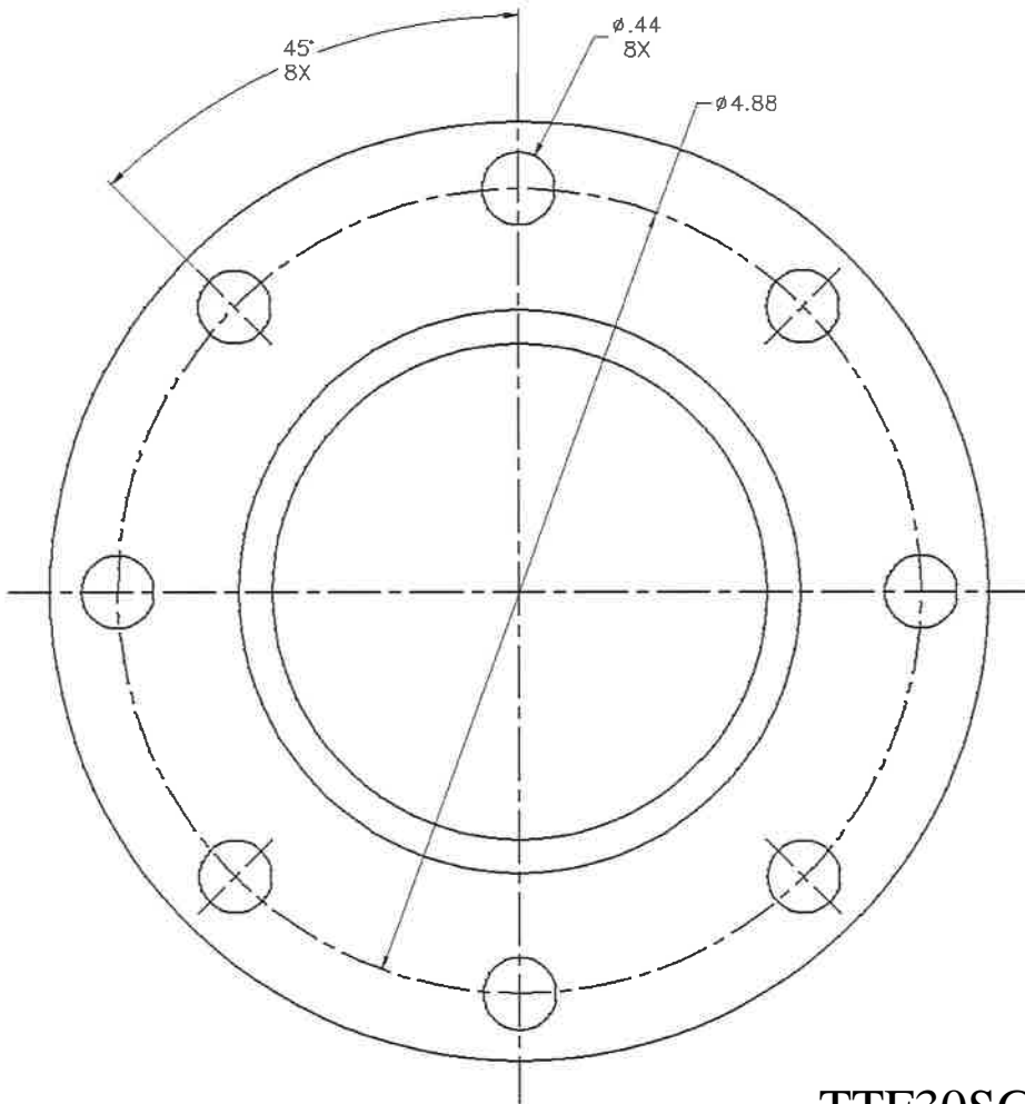
TTF30SG 3" TTMA Flange Solid Acrylic 50 psi max
