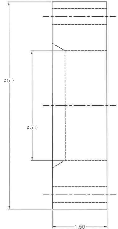
TTF30SG 3" TTMA Flange Solid Acrylic 50 psi max
